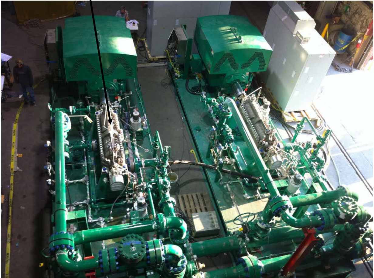
MODULAR WATER INJECTION PACKAGE
